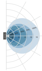
Wall mounting pattern(Unit:m) Suggested installation height: 1-1.8m
